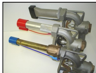
EBW and Morrison 1" round nozzle spouts
