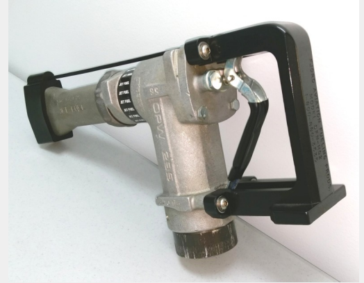
SFN-HG2 Handle Guard for the 1½” OPW 295SA and 295SAJ Series Overwing Fueling Nozzles
