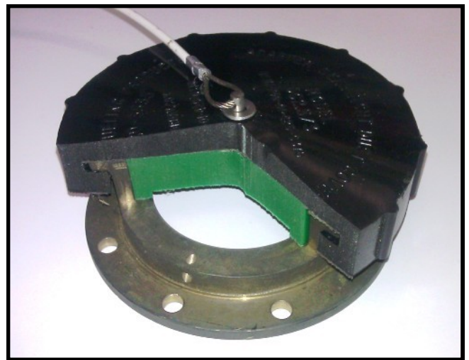
DC 2.5/3-P (cut away view)
